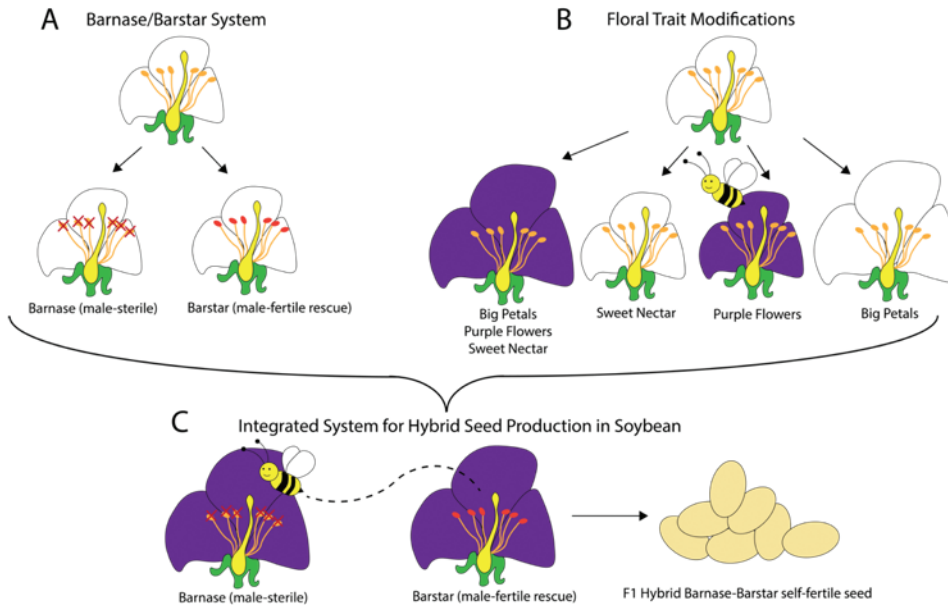
Figure 1. Integration of (A) Barnase/Barstar system for male-sterile lines and (B) floral trait modifications to create (C) hybrid soybean seed.
