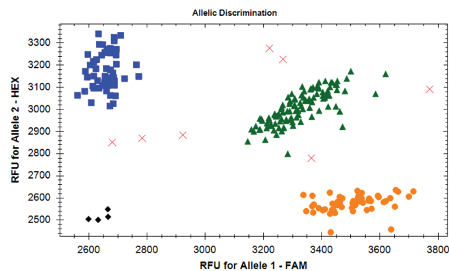
Figure 1. Selection of high protein lines with DNA markers developed at University of Georgia.
