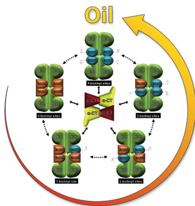
Figure 1. Reducing the level BADC protein in developing soybean seeds is hypothesized to increase ACCase activity, resulting in more seed oil production. BADC usually competes with BCCP, a required ACCase subunit, limiting activity of the enzyme.
