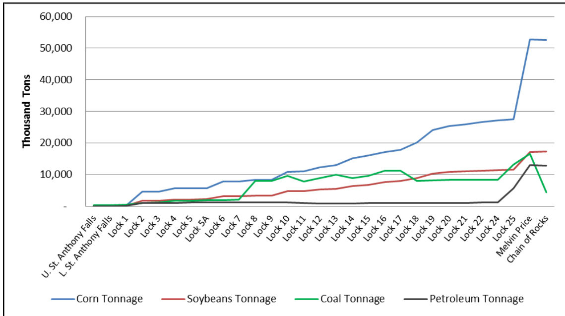
Figure 6. Commodity Volumes (Both Directions) at Upper Mississippi River Locks for 2008–2010.
