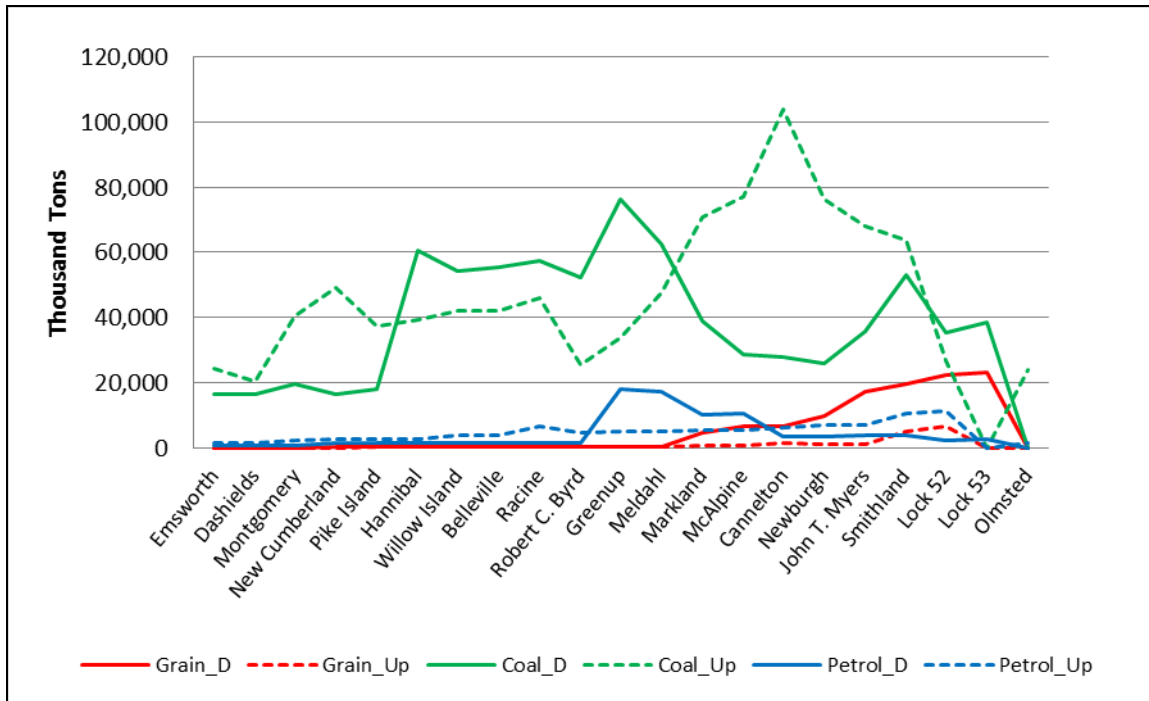
Figure 12. Commodity Movements through Ohio River Locks during 2008–2010.
