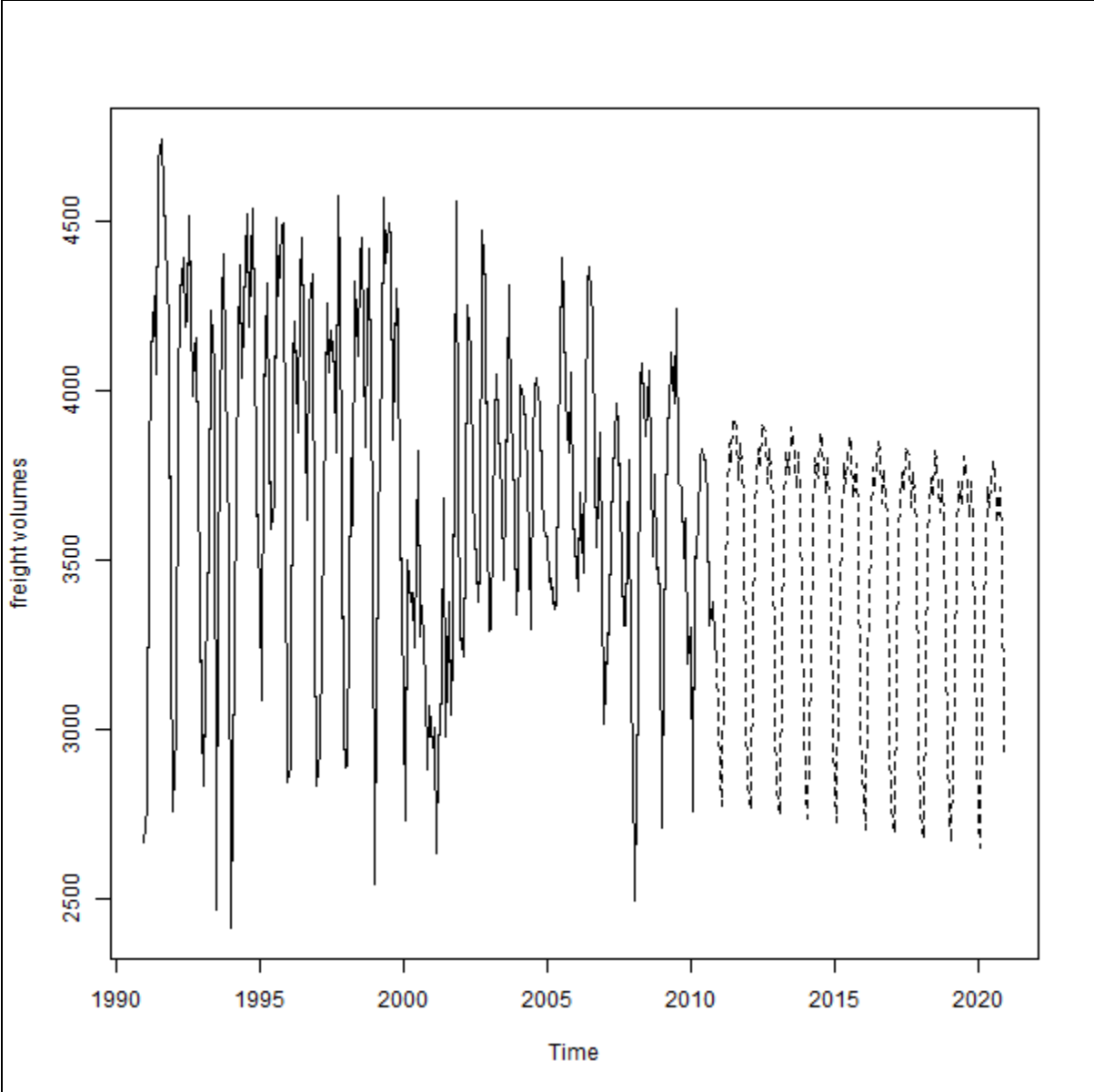
Figure 17. Forecasts Based on Regression Model.
