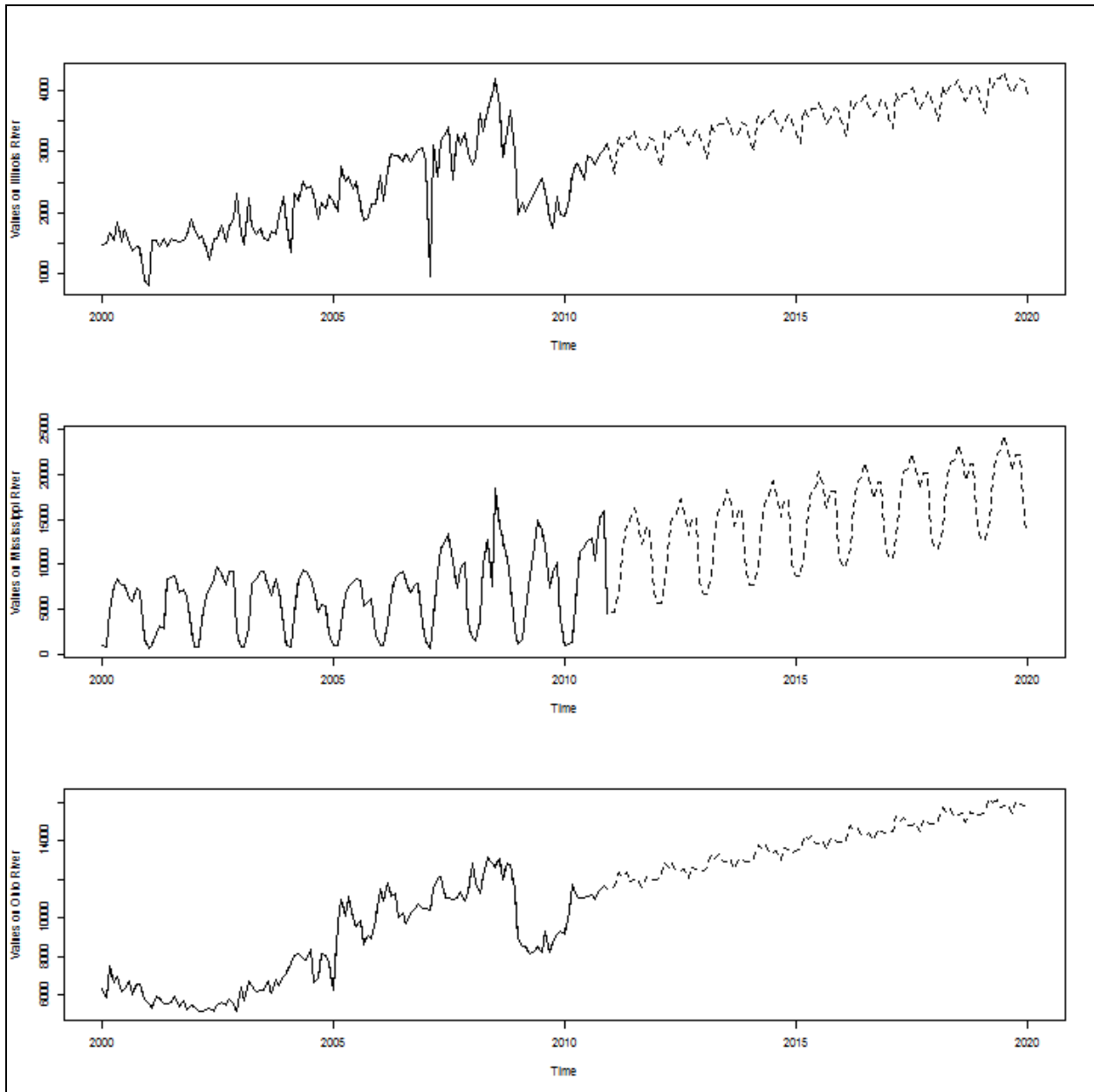
Figure 19. Forecasting of Freight Values.
