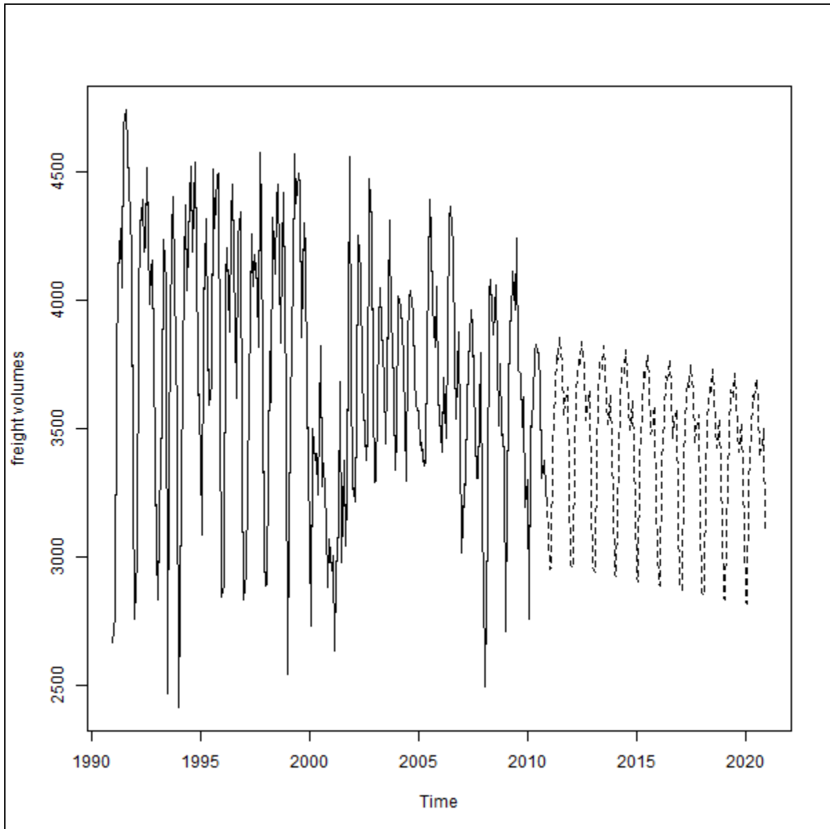
Figure 16. Ten-Year Forecasting Based on ARIMA Model.
