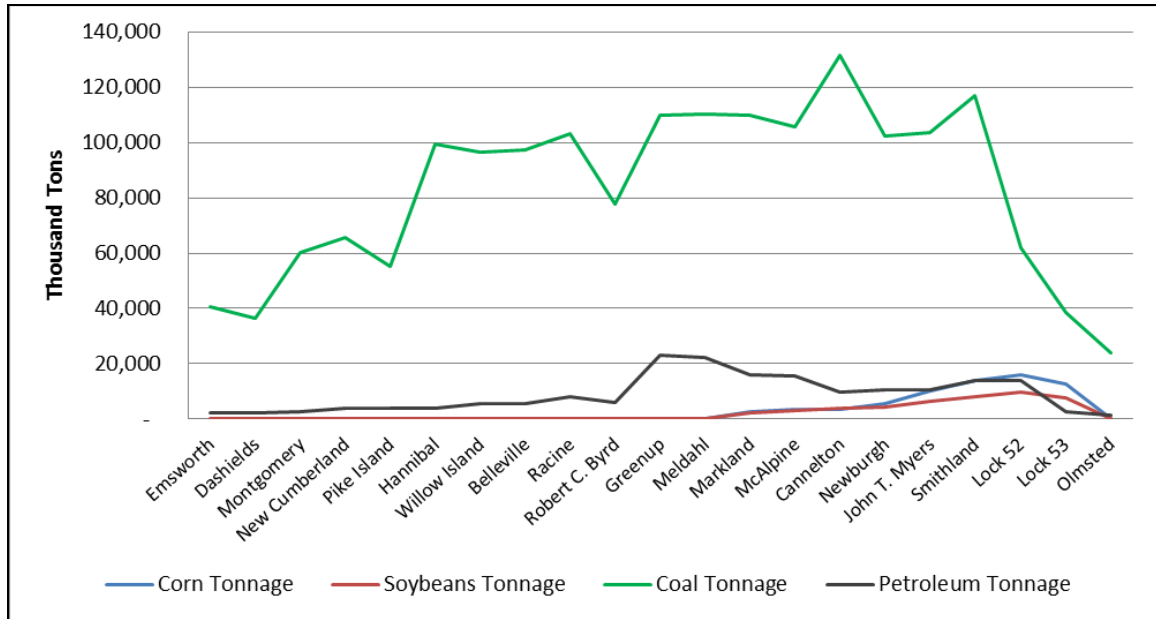
Figure 8. Commodity Volumes (Both Directions) at Ohio River Locks for 2008–2010.
