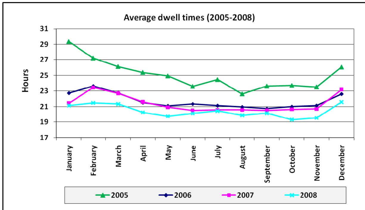
Figure 9. Average Terminal Dwell Times (2005–2008).
