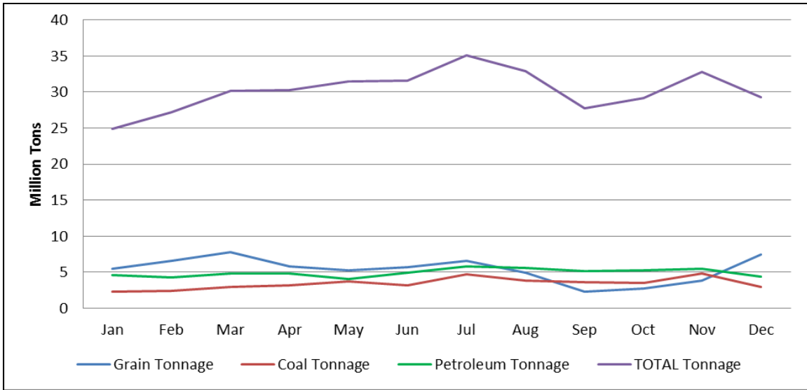
Figure 3. Total Volume of Commodity Flows in Both Directions on Illinois River during 2008–10.
