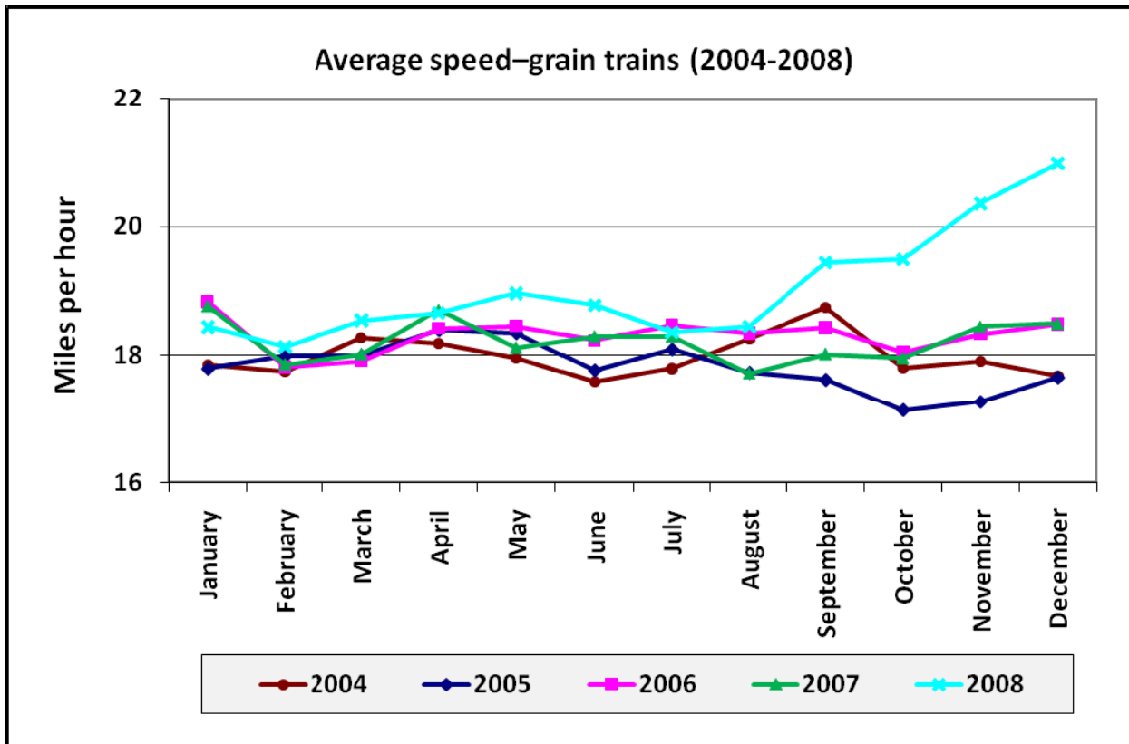
Figure 8. Average Speed—Grain Trains (2004–2008).
