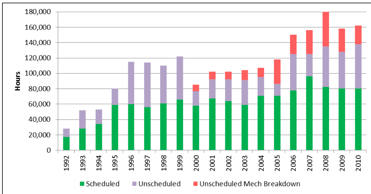
Figure 2. Hours of Lock Outages by Year and by Type of Outage.
