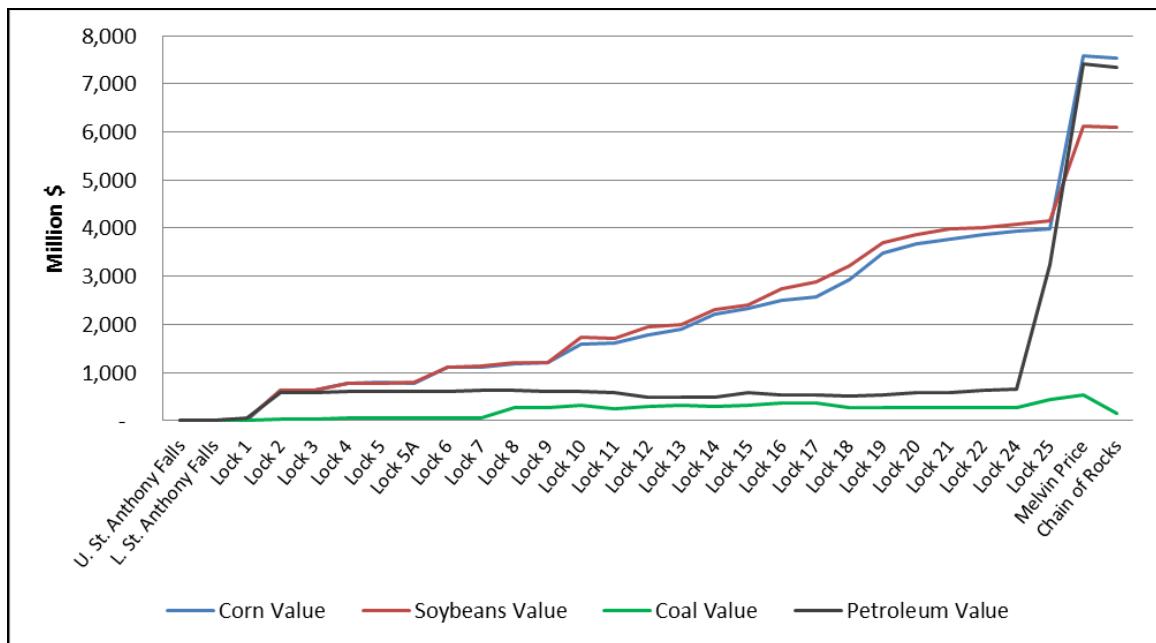
Figure 7. Commodity Values (Both Directions) at Upper Mississippi River Locks for 2008–2010.
