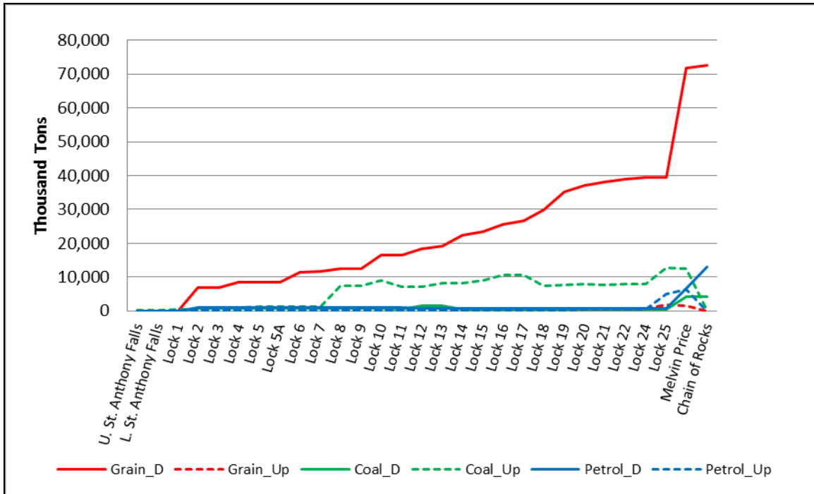
Figure 11. Commodity Movements through Upper Mississippi River Locks during 2008–2010.
