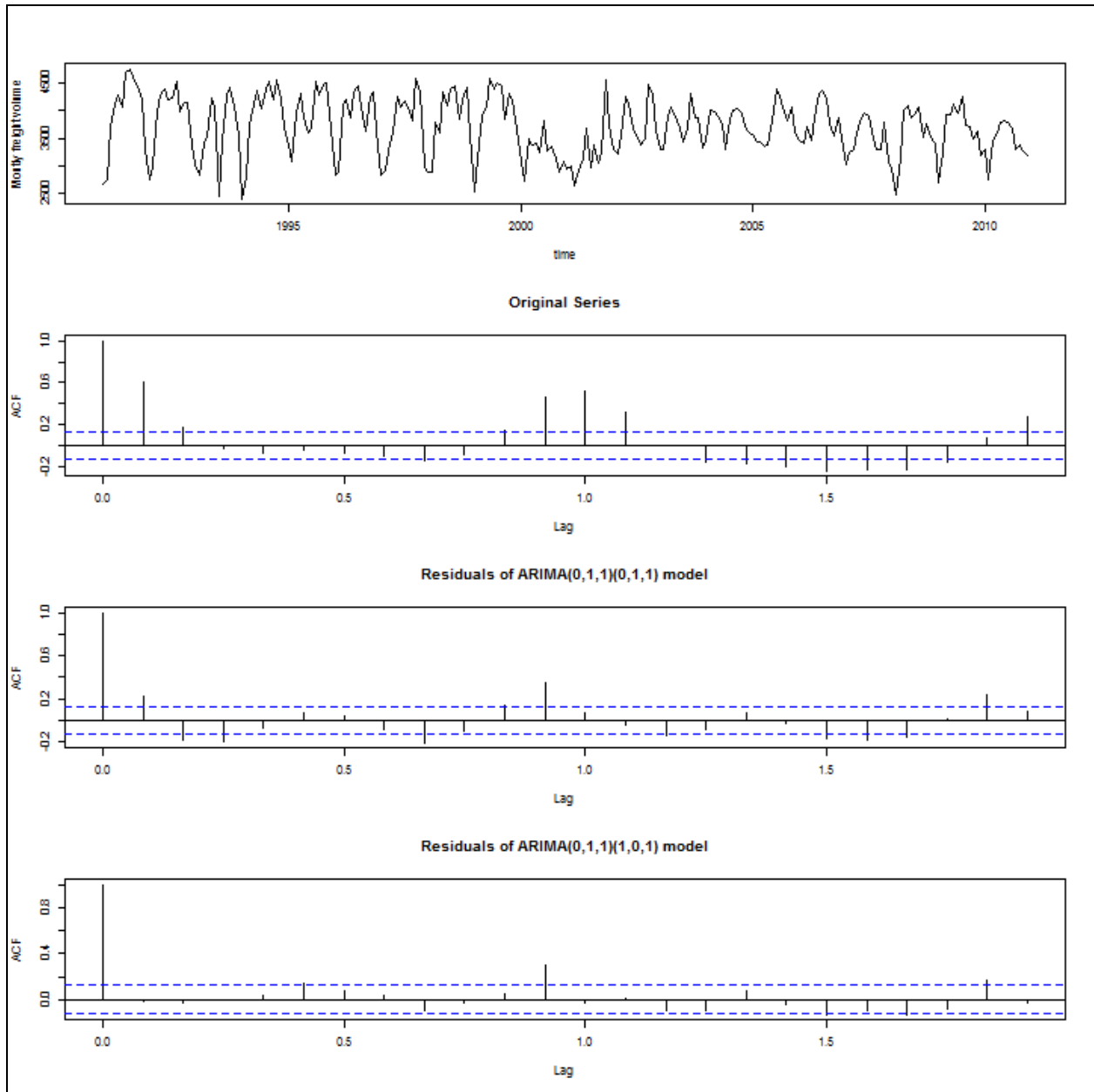
Figure 14. Time Series Analysis of Freight Volumes.
