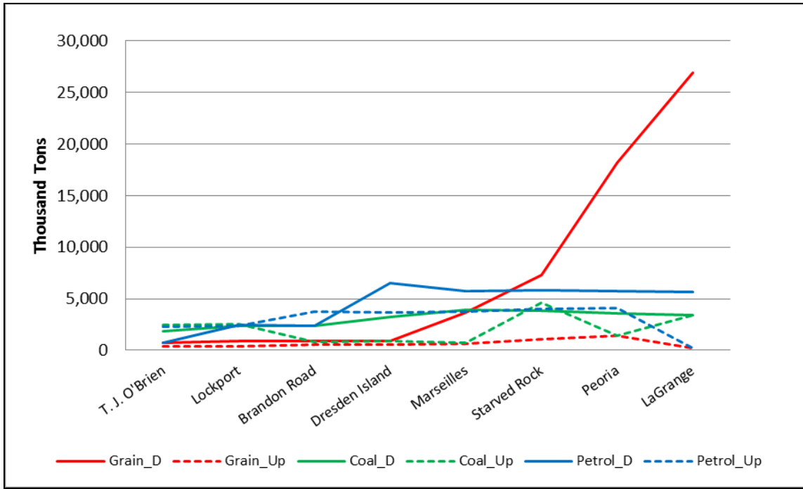
Figure 10. Commodity Movements through Illinois River Locks during 2008–2010.
