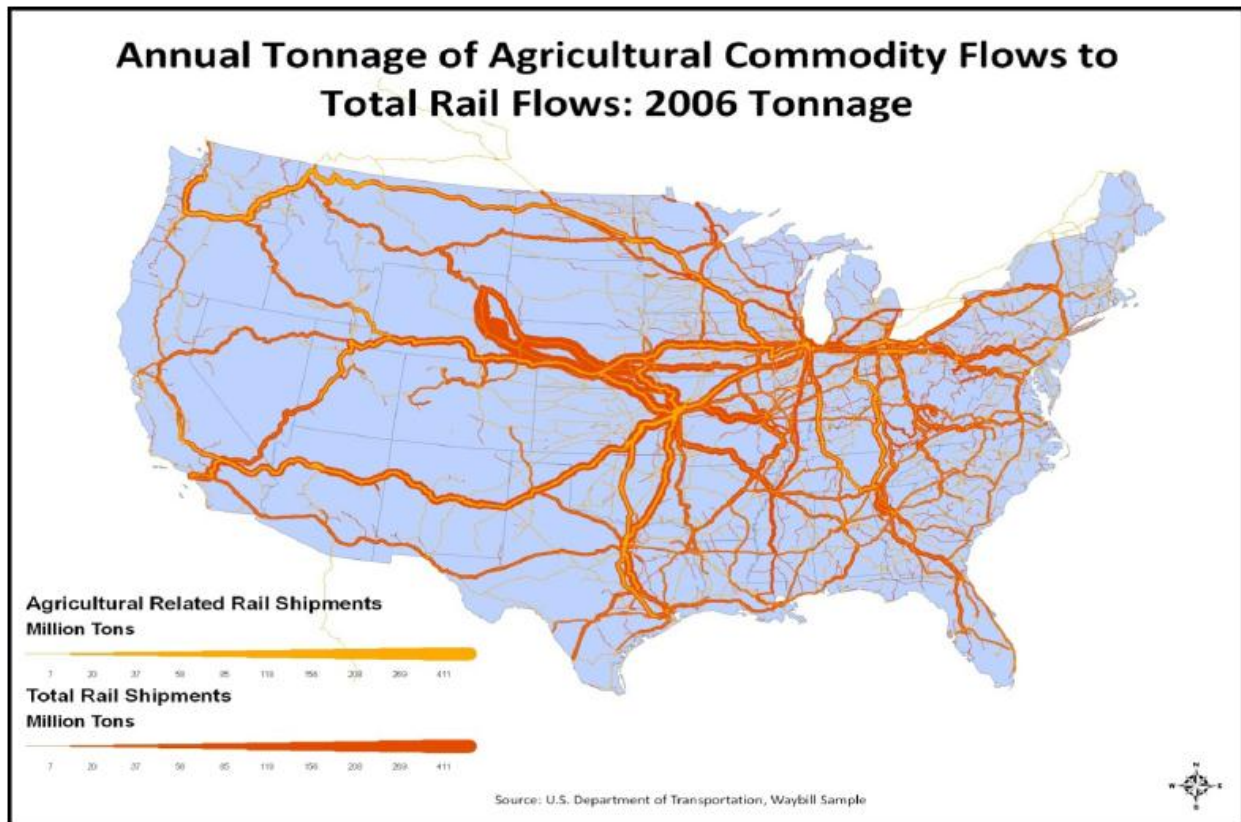
Figure 6. Rail Commodity Flows (2006).
