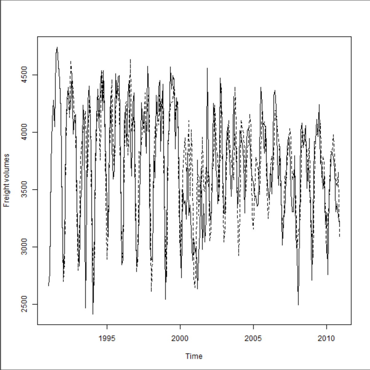
Figure 15. Estimated Freight Volumes (Dotted) vs. Observed Volumes (Solid).
